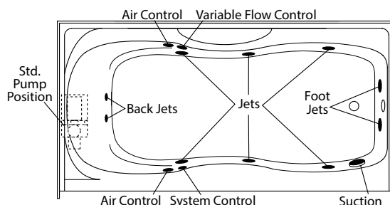
InVigor Hydrotherapy System
