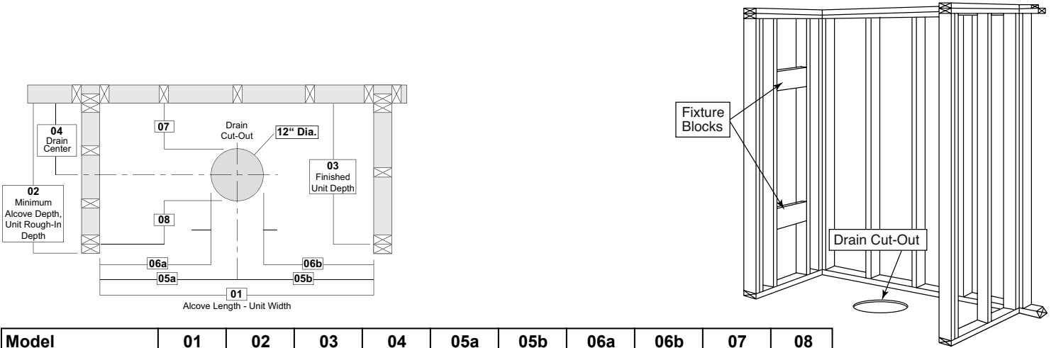
Illustration 1b - Center Drain, Unit Dimension & Alcove Framing Guidelines (dimensional tolerance +0 / -3/8")
