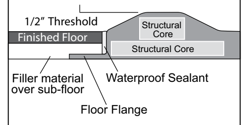
Illustration 9b - SHFW-6235 Floor Flange Detail
