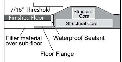
Illustration 9c - SHMD Floor Flange Detail
