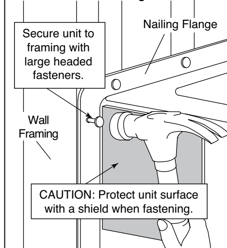
Illustration 6 - Securing Unit
