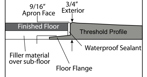
Illustration 9c - SHMD Floor Flange Detail
