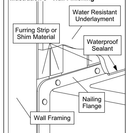
Illustration 8 - Wall Finishing
