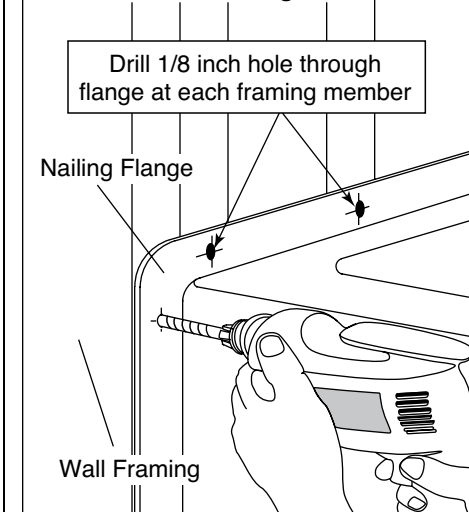
Illustration 5 - Securing Unit
