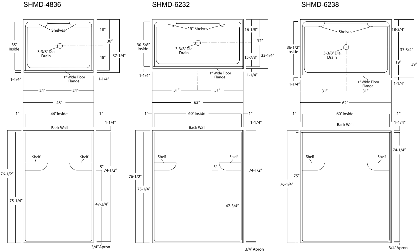
Illustration 1b - Minimal Threshold, Center Drain, Unit Dimension & Alcove Framing Guidelines (dimensional tolerance + / -1/8")
