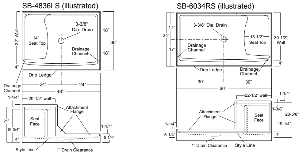
Illustration 1c - Center Drain, Unit Dimension & Alcove Framing Guidelines (dimensional tolerance +0 / -1/8")
