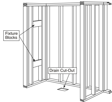
Illustration 1c - Center Drain, Unit Dimension & Alcove Framing Guidelines (dimensional tolerance +0 / -1/8")
