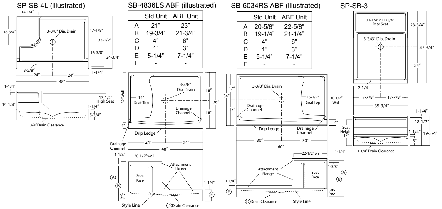
Illustration 1c - Center Drain, Unit Dimension & Alcove Framing Guidelines (dimensional tolerance +0 / -1/8")
