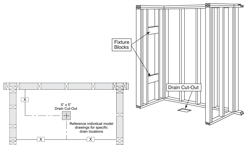
Illustration 5 - Securing Unit
