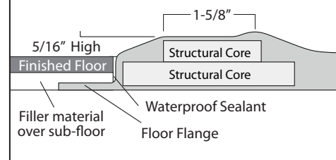
MDWX Contoured Threshold Profile
